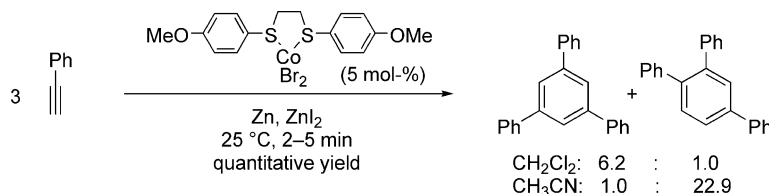
Scheme 1. Benchmark ligands for the regioselective cyclotrimerisation of phenylacetylene.
