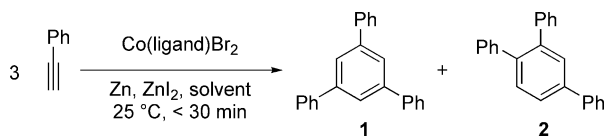
Scheme 2. Optimisation of disulfide ligands in the cobalt-catalysed cyclotrimerisation in different solvents.
